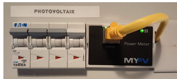
Figure 3: The my-PV Power Meter is mounted in the distribution cabinet directly after the utility meter.
